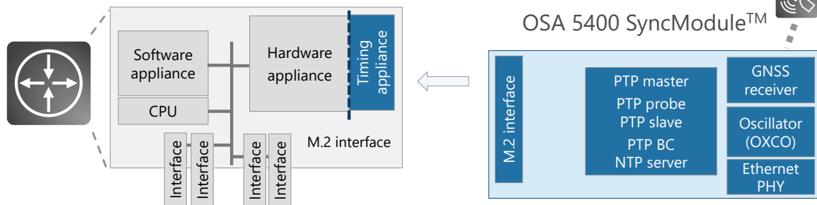
Generic architecture of a network device
